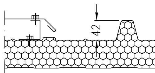
DETAIL PUNKT "A"
